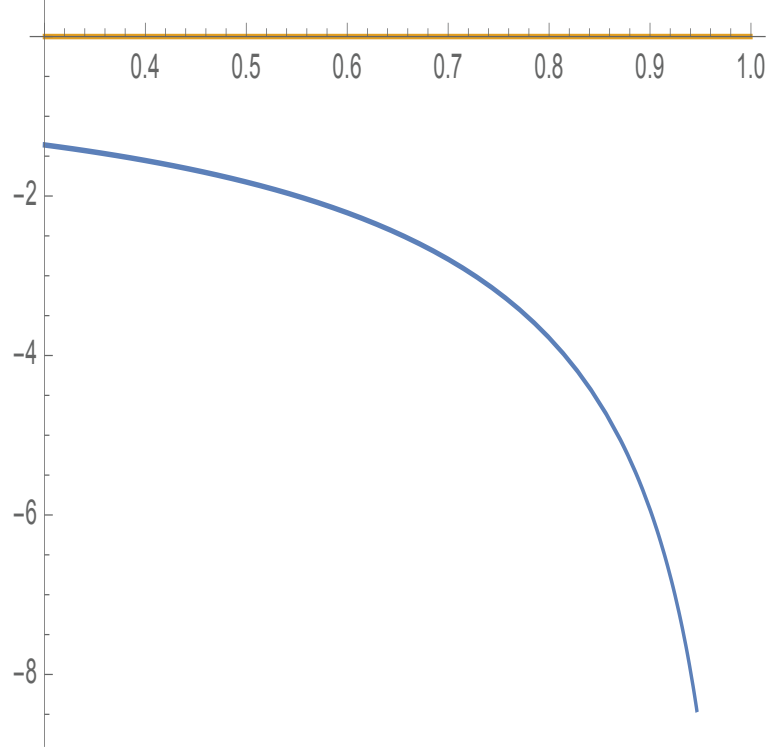
FIGURE 2. The graph of the function I(\kappa) . Note that I(\kappa) < 0, \kappa \in (0.98, 1)
